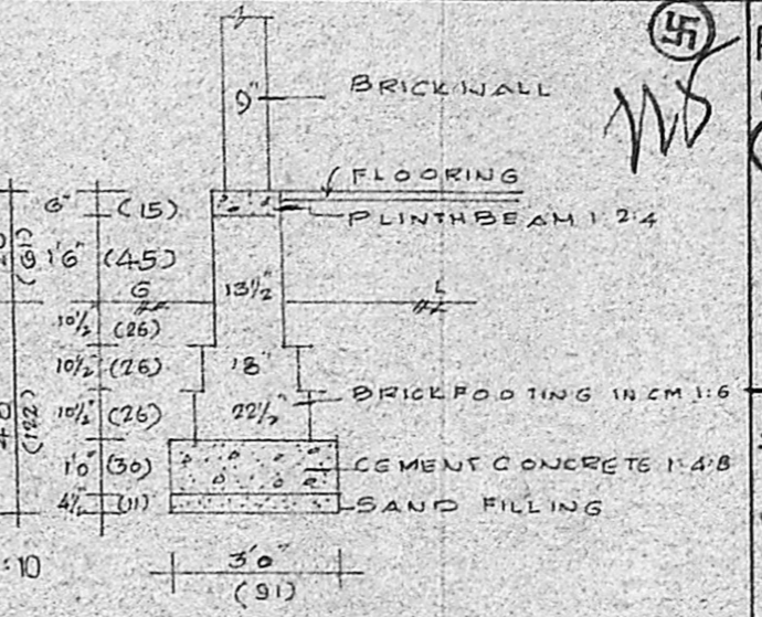
FOUNDATION DETAILS
